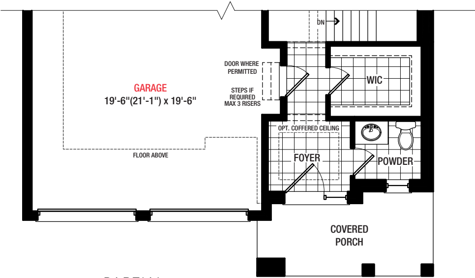
PARTIAL GROUND FLOOR B
