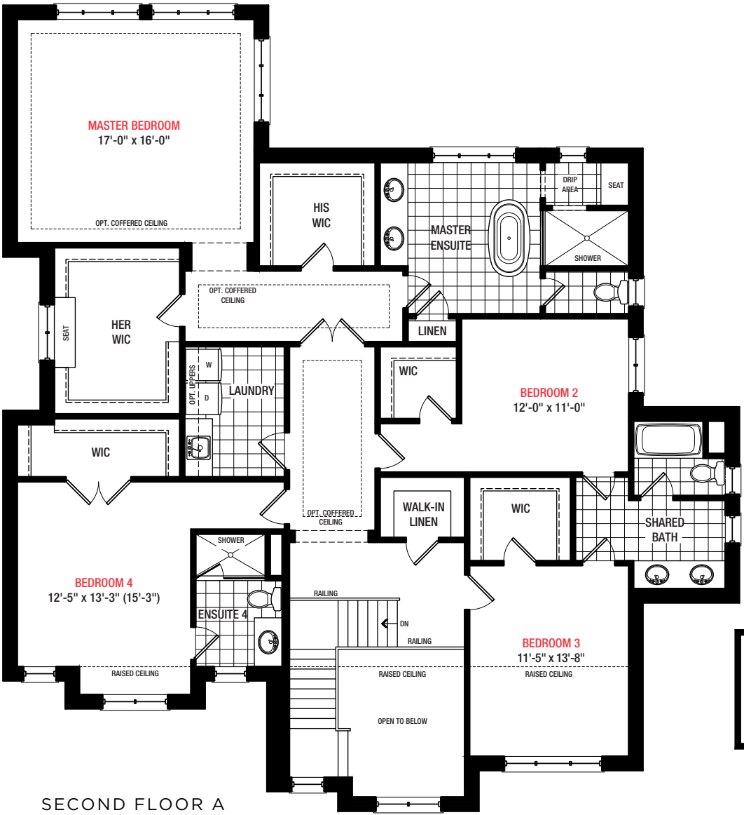
SECOND FLOOR A
