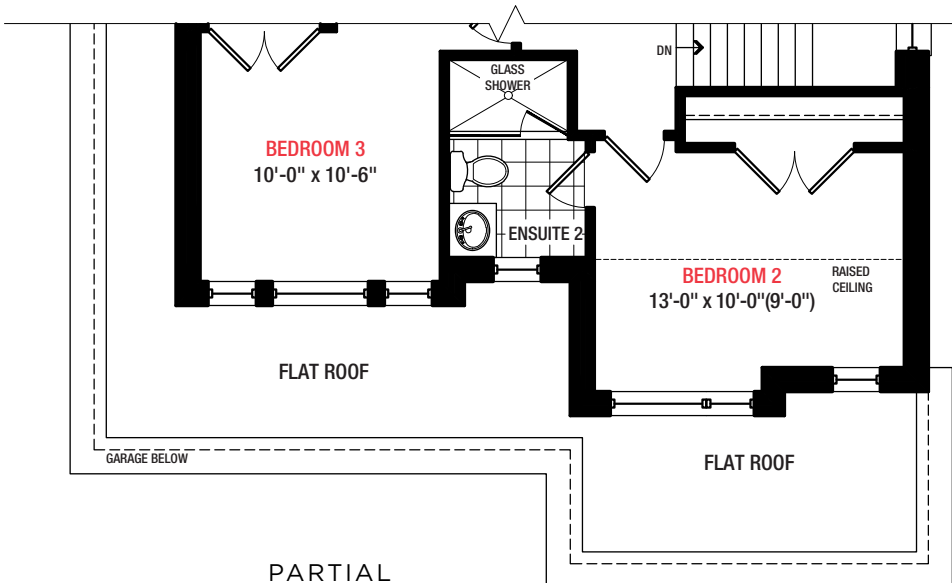
PARTIAL SECOND FLOOR B
