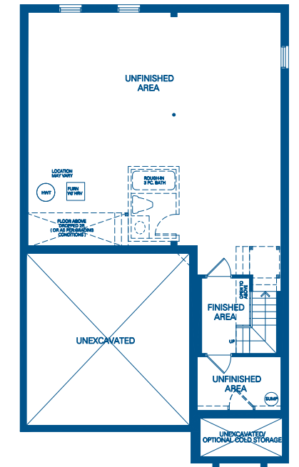
BASEMENT A
