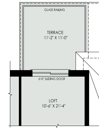
SECOND FLOOR PLAN OPTIONAL TERRACE ELEV. 'A'
