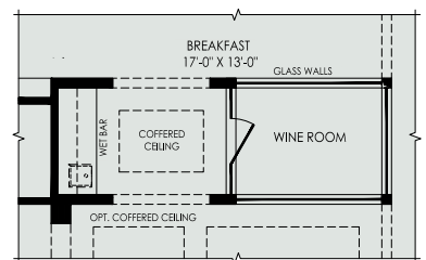
GROUND FLOOR PLAN OPTIONAL WINE ROOM ELEV. 'A'
