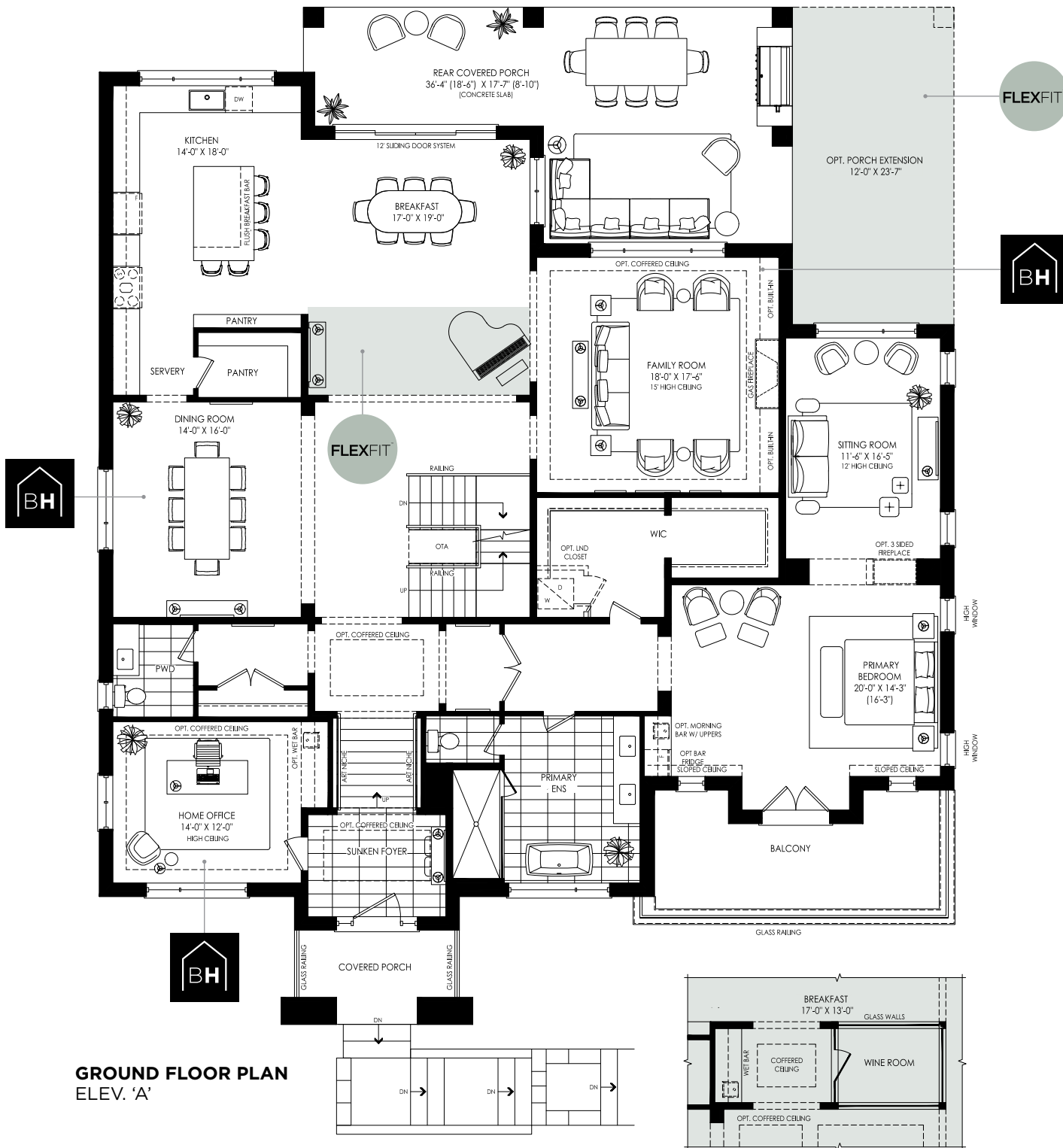
GROUND FLOOR PLAN OPTIONAL WINE ROOM ELEV. 'A'
