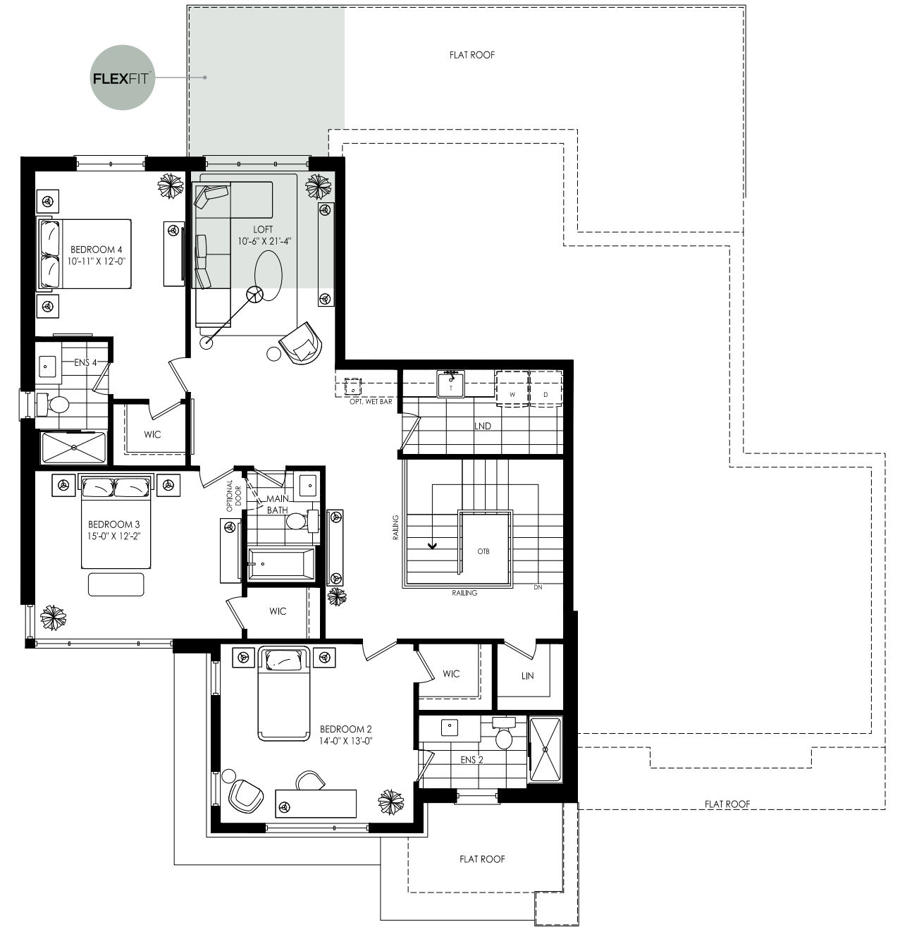
SECOND FLOOR PLAN ELEV. 'A'
