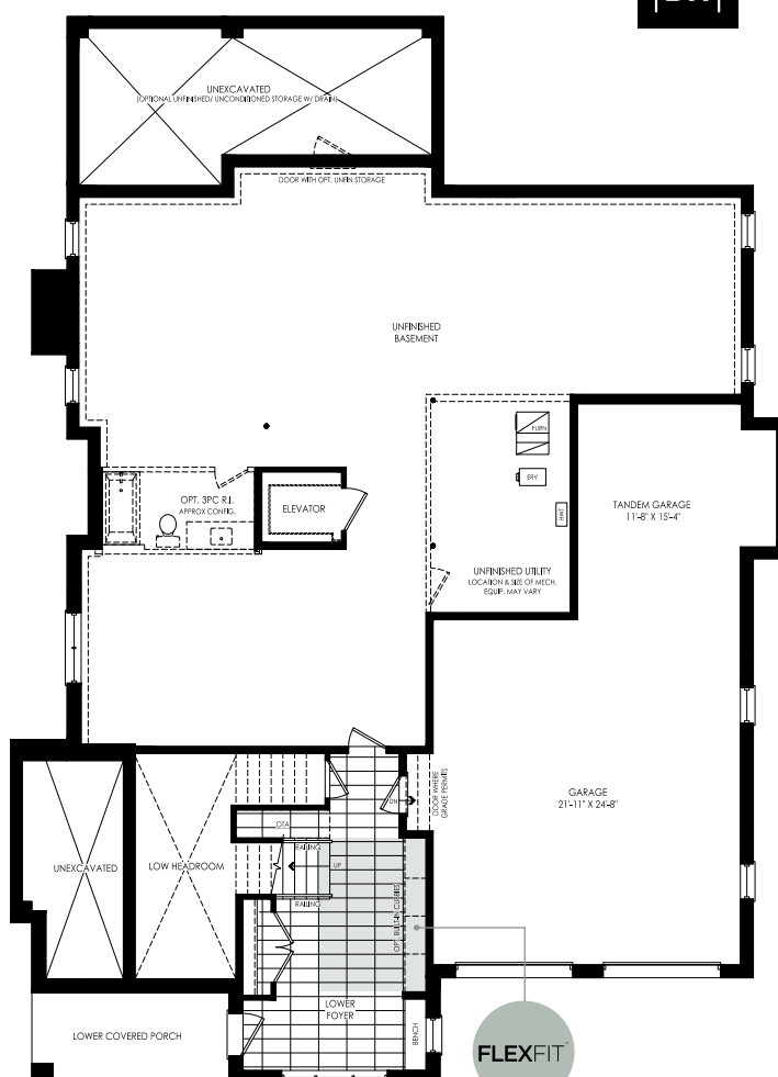
BASEMENT FLOOR PLAN W/ ELEVATOR ELEV. 'A'
