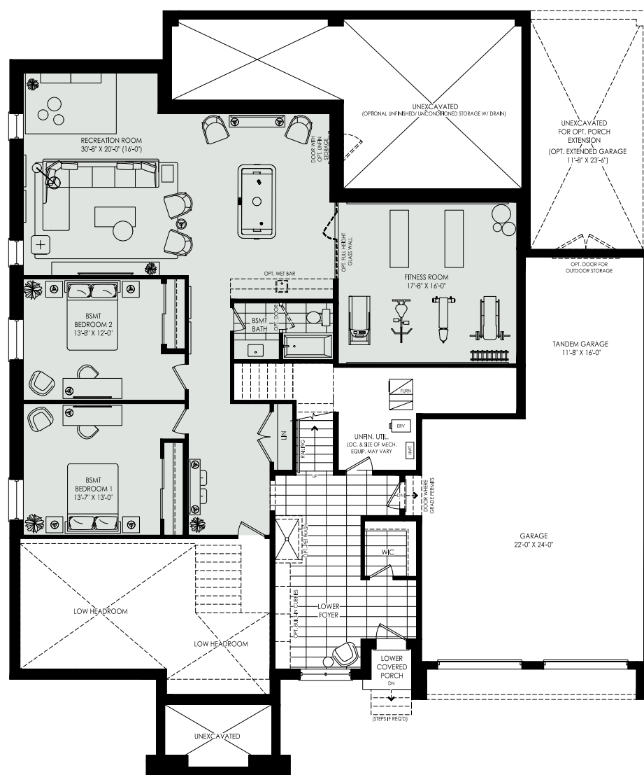
OPTIONAL FINISHED BASEMENT FLOOR PLAN ELEV. 'A'
