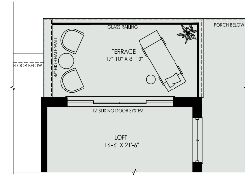
SECOND FLOOR PLAN OPTIONAL TERRACE ELEV. 'A'
