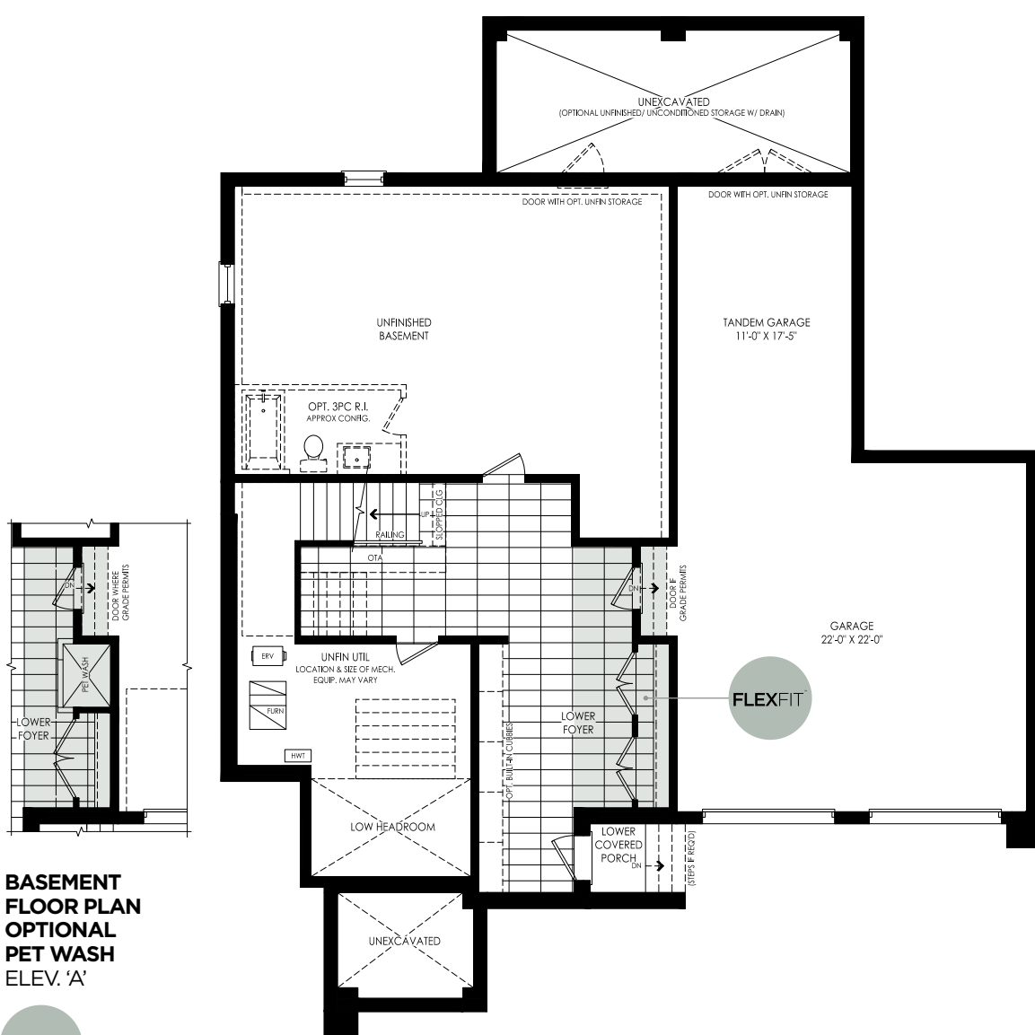
BASEMENT FLOOR PLAN ELEV. 'A'
