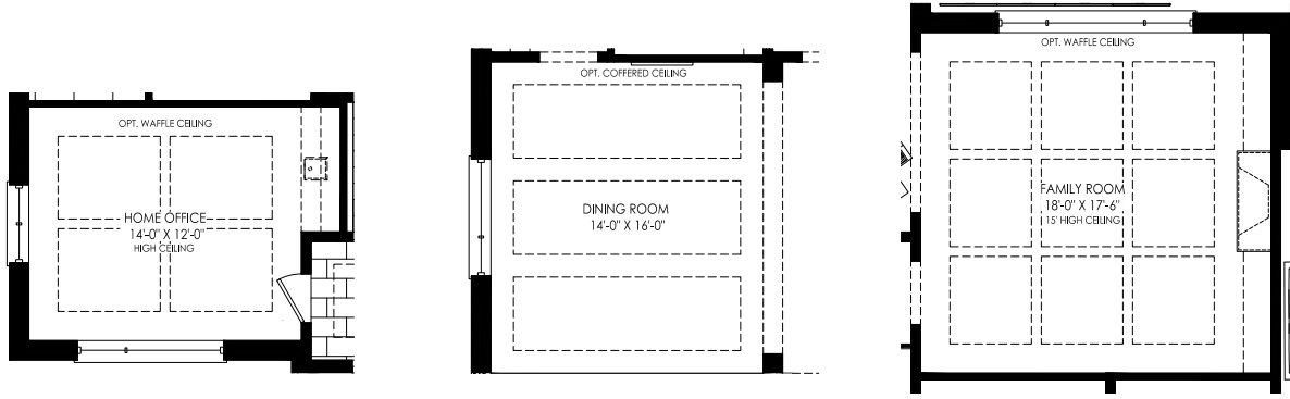
GROUND FLOOR PLAN OPTIONAL CEILING TREATMENTS ELEV. 'A'
