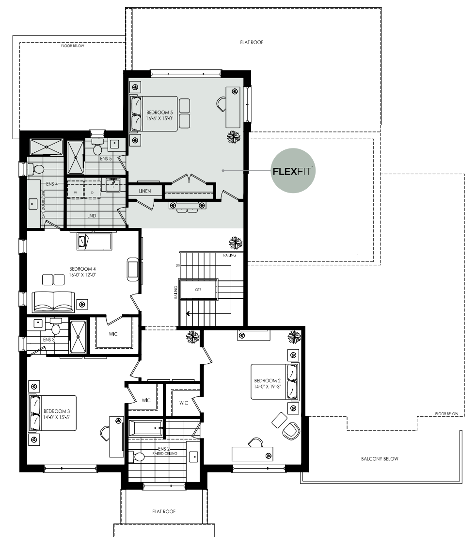
SECOND FLOOR PLAN OPTIONAL 5 BEDROOM PLAN ELEV. 'A'
